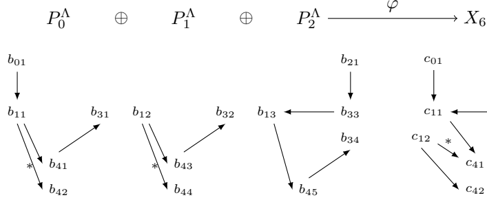
FIGURE 13. The projective cover of E
