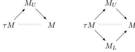
FIGURE 21. The mesh ending at an indecomposable object in \mathcal{T} . The diagram on the left indicates the case where M is on the border of \mathcal{T} .
