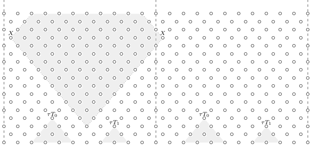
FIGURE 8. Proof of Proposition 3.7: the shaded region indicates part of (one copy of) the diamond-shaped region D_X . In this case, u_X does not factor through \text{add}(\tau T_{\mathcal{T}}) .
