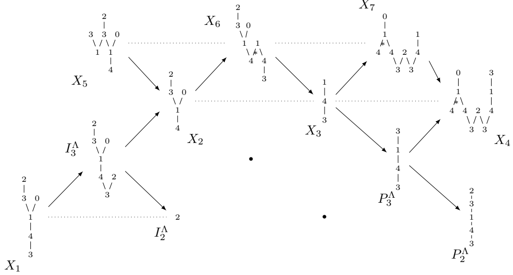
FIGURE 16. Part of the AR-quiver of \Lambda -mod
