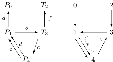
FIGURE 12. Maps between indecomposable projective KQ -modules and the quiver with relations of \text{End}_{\mathcal{C}}(T)^{\text{opp}} .
