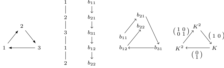
FIGURE 1. A quiver Q , a Q -coloured quiver, together with the redrawing according to Remark 1.2 and the corresponding representation of Q .
