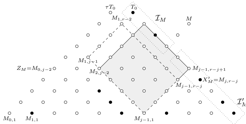
FIGURE 24. Part of the proof of Lemma 7.4 in the case r = 11 , j = 7 . The dotted rectangles show \mathcal{I}_M and \mathcal{I}'_M . Since V \in \mathcal{W}_{T_0} , we have \text{Hom}(\tau^{-2}Z_M, V) \neq 0 if and only if V lies in the shaded rectangle. Since \text{Ext}(V, X'_M) = 0 , V cannot lie in the dashed rectangle. By the definition of X'_M , V cannot lie in the part of \mathcal{I}'_M above X'_M . Hence \text{Hom}(Z_M, \tau^2 V) \neq 0 if and only if V \in \mathcal{I}_M \setminus \{T_0\} .
