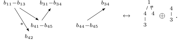
FIGURE 15. The kernel of the projective cover of X_6
