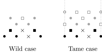
FIGURE 20. \tau -rigid, rigid and Schurian \Lambda -modules in part of a wild example (left hand diagram). In the right hand diagram we recall the \tau -rigid, rigid and Schurian modules from the tame case in Example 1.6 shown in Figure 9.
