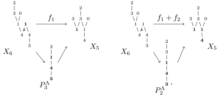
FIGURE 18. Rigidity of X_5 .
