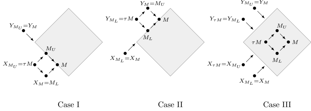
FIGURE 23. Proof of Lemma 7.2. The shaded region is the region D .
