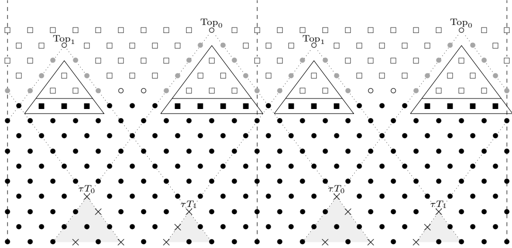
FIGURE 10. Schurian and rigid \Lambda -modules for a particular choice of tilting module T . The notation is as in Figure 9.
