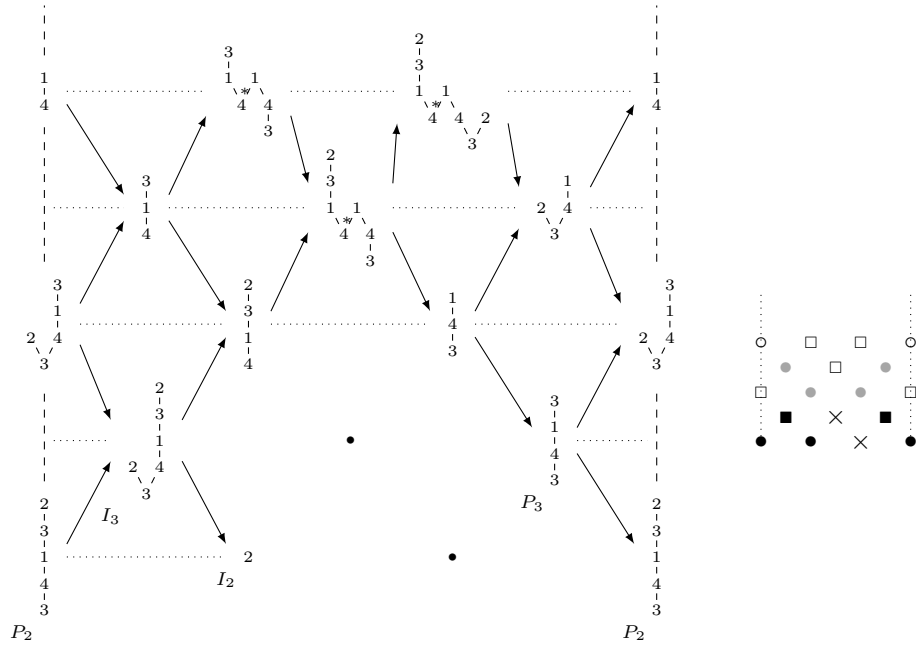
FIGURE 9. The left hand diagram shows part of the AR-quiver of \Lambda\text{-mod} . The right hand diagram shows the same objects. The symbol for a module is circular if it is Schurian, filled-in with gray if it is rigid but not \tau -rigid, and filled-in with black if it is \tau -rigid. The symbol \times represents a gap in the AR-quiver (corresponding to an indecomposable direct summand of \tau T )
