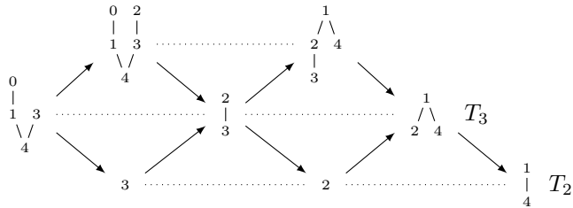
FIGURE 11. Part of the AR-quiver of KQ -mod.
