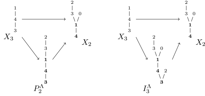
FIGURE 17. Rigidity of X_2 and X_3 .
