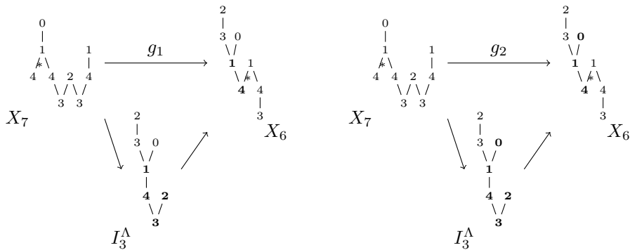
FIGURE 19. Rigidity of X_6 .
