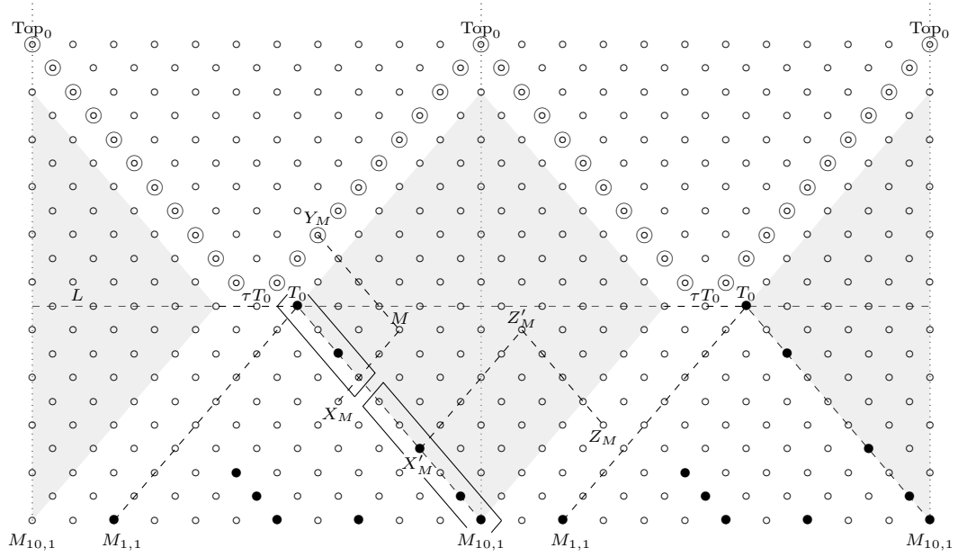
FIGURE 22. Here the rank of the tube is 11. The region D is indicated by the shaded area. The filled-in circles indicate the indecomposable direct summands of T , and the double circles indicate the elements of \mathcal{H}_0 . The line L divides the region D into two and \mathcal{S}_0 consists of the vertices in D on and above the line. The upper boxed region is \mathcal{I}_M (see (7.2)) and the lower boxed region is \mathcal{I}'_M (see (7.8)).
