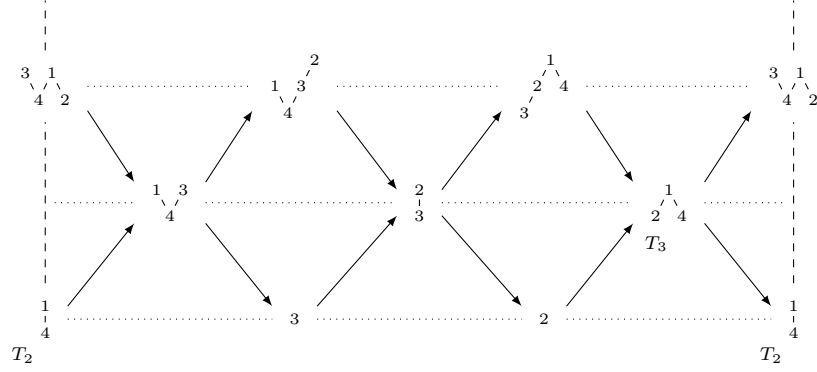
FIGURE 2. Part of the AR-quiver of KQ\text{-mod} , where Q is the quiver in (1.3).
