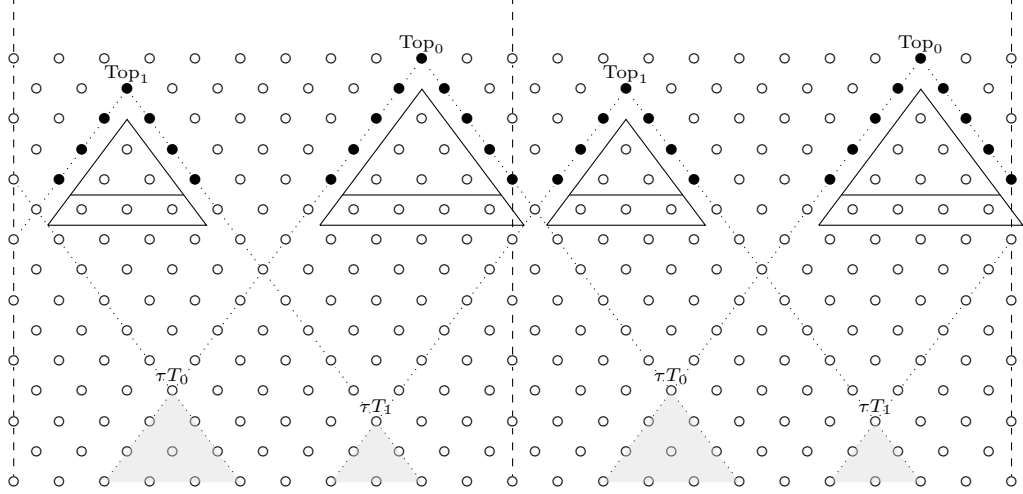
FIGURE 6. The wings \mathcal{W}_{\tau T_k} shown as shaded regions in two copies of \mathcal{T} in the case r = 11 . The elements in the \mathcal{H}_k are drawn as filled dots. The elements in the regions \mathcal{R}_k and \mathcal{S}_k are enclosed in triangles.
