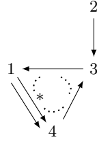
FIGURE 3. The endomorphism algebra \text{End}_{\mathcal{C}}(T)^{\text{opp}} for the tilting module in Example 1.6.
