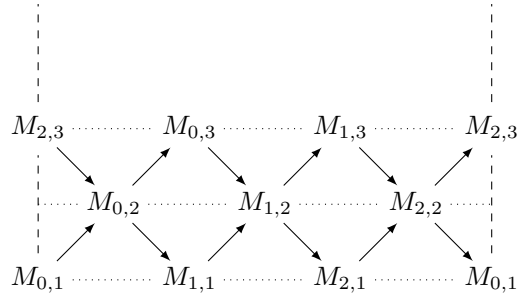
FIGURE 4. The AR-quiver of a tube of rank 3
