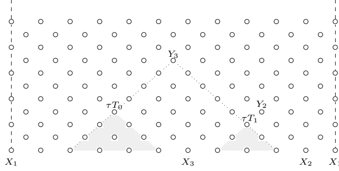
FIGURE 7. Proof of Proposition 3.4. For the quasisimple module X_1 , we take Y = X_1 ; for the module X_2 , we take Y = Y_2 , and for the module X_3 , we take Y = Y_3 .
