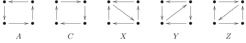
FIGURE 28. Four-vertex quivers
