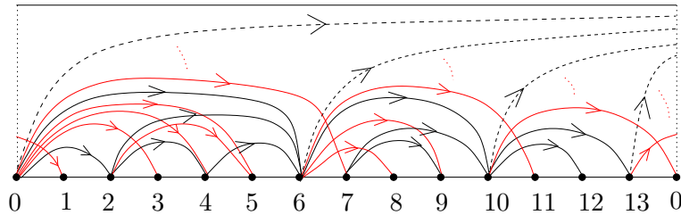
FIGURE 14. The torsion-free part, \mathcal{F}_U = \text{Cogen } U \cap \mathbf{T} , of the torsion pair corresponding to U . The arcs not in \text{add } U are drawn in red. The dashed arcs are the indecomposable summands of U which are not of finite length (and thus not in \mathcal{F}_U ). The arcs \pi_{14}([0, j]) for j \geq 8 , \pi_{14}([6, j]) for j \geq 12 , \pi_{14}([10, j]) for j \geq 15 and \pi_{14}([13, j]) for j \geq 16 have been omitted for clarity.
