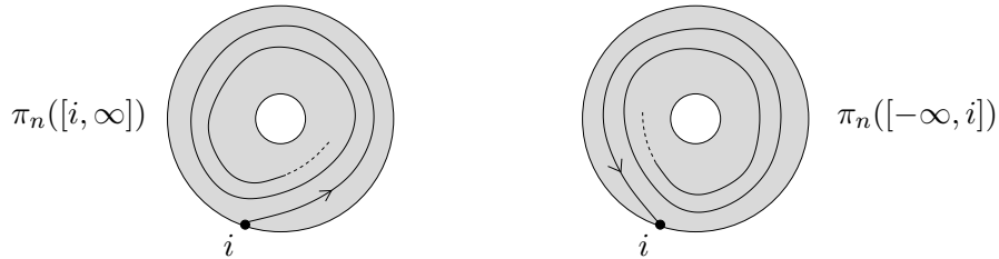
FIGURE 7. Infinite arcs in \mathbb{A}(n) .
