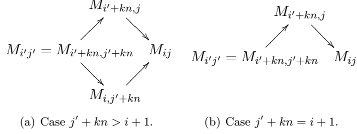
FIGURE 10. Objects and paths in the Auslander-Reiten quiver of \mathbf{T} corresponding to an intersection in \mathbb{U}(n) between arcs [i, j] and [i' + kn, j' + kn] .
