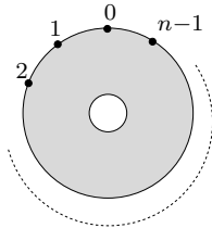
FIGURE 4. An annulus with n marked points on its outer boundary.
