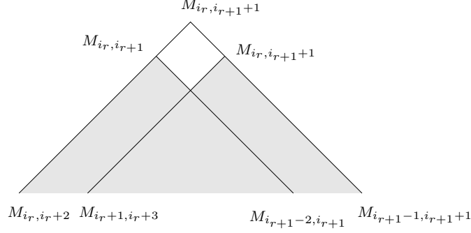
FIGURE 9. A wing \mathcal{W}_{i_r, i_{r+1}+1} .
