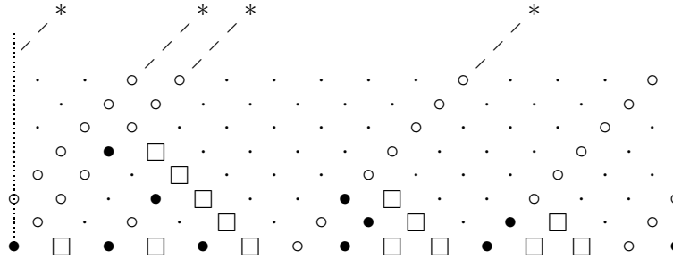
FIGURE 15. The AR-quiver of the tube, showing the indecomposable summands of U ( \bullet or * ), \text{ind}(\mathcal{T}_U) ( \square ) and \text{ind}(\mathcal{F}_U) ( \circ or \bullet ). The Prüfer direct summands of U are shown (symbolically) at the top of the diagram as asterisks.
