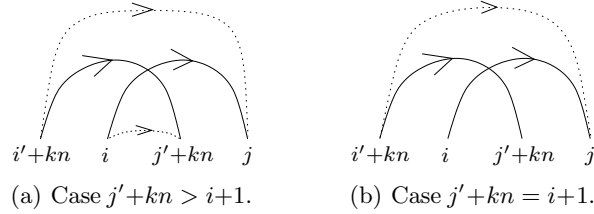
FIGURE 11. Non-split extensions in \mathbf{T} represented geometrically.
