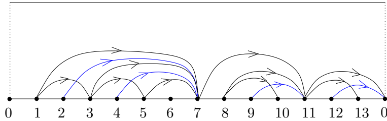
FIGURE 13. The torsion part, \mathcal{T}_U = \tau^{-1}(\text{Gen } U \cap \mathbf{T}) , of the torsion pair corresponding to U . The arcs corresponding to indecomposable objects not in \tau^{-1}(\text{add } U \cap \mathbf{T}) are drawn in blue.
