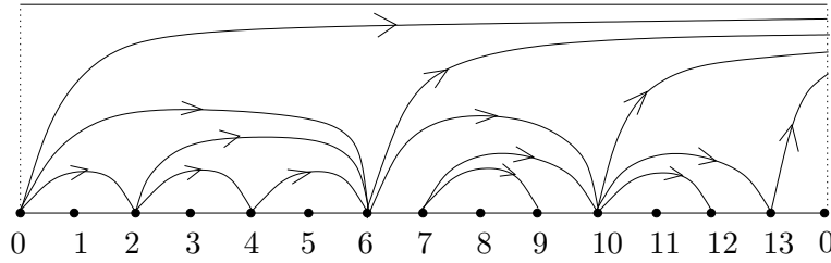
FIGURE 12. The maximal rigid object U
