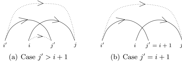
FIGURE 2. Non-split extension
