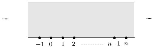
FIGURE 5. The universal cover of the annulus in Figure 4.
