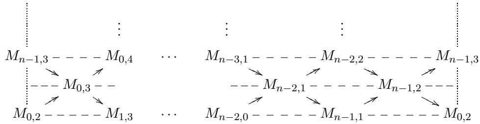
FIGURE 3. The AR-quiver of \mathbf{T}_n
