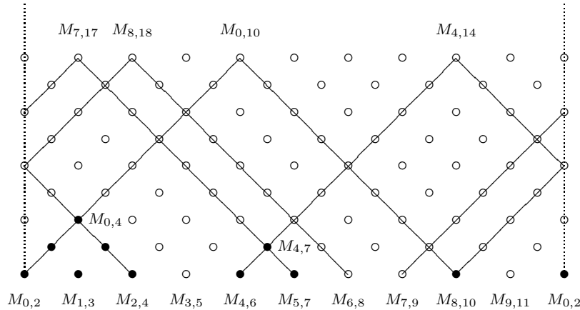
FIGURE 8. The indecomposable objects in the intersection of the four wings \mathcal{W}_{0,10}, \mathcal{W}_{4,14}, \mathcal{W}_{7,17} and \mathcal{W}_{8,18} in a tube of rank 10 corresponding to a maximal rigid object of Prüfer type. The objects lying in the intersection are indicated by filled-in circles. The intersection coincides with \mathcal{W}_{0,4} \amalg \mathcal{W}_{4,7} \amalg \mathcal{W}_{8,10} (note that the wing \mathcal{W}_{i_3, i_4} = \mathcal{W}_{7,8} is zero).
