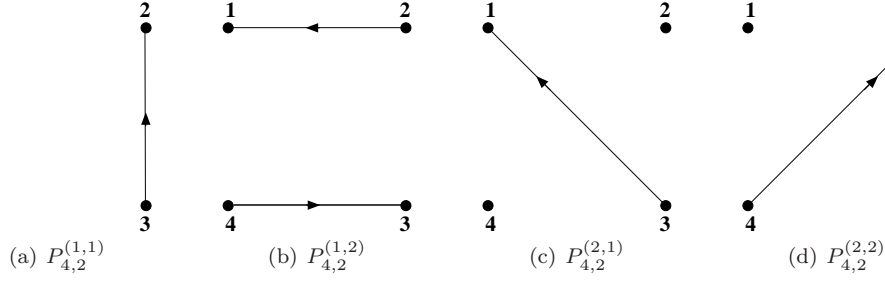
Figure 5: The strictly period 2 primitives for 4 nodes.
