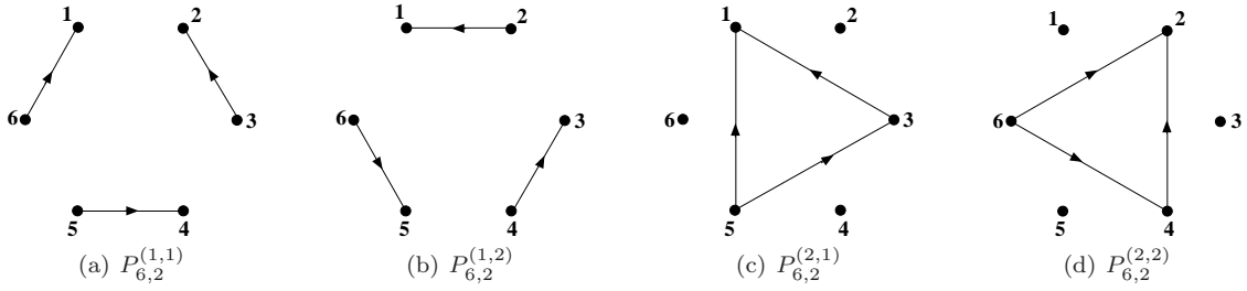
Figure 6: The period 2 primitives for 6 nodes
