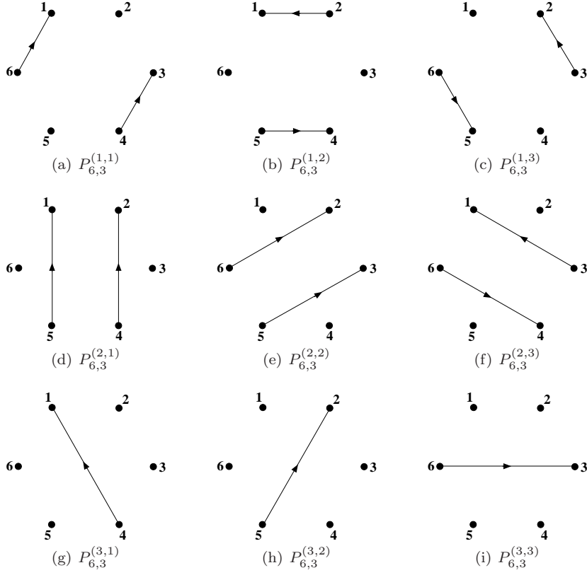
Figure 8: The period 3 primitives for 6 nodes.
