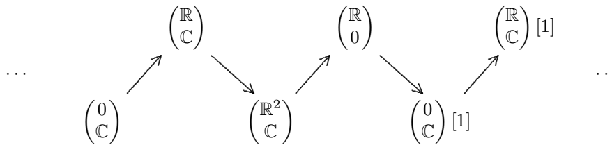
FIGURE 12. The AR-quiver of D^b(H)
