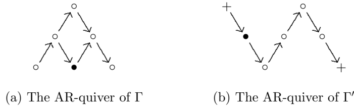
FIGURE 15. The AR-quivers of \Gamma and \Gamma'
