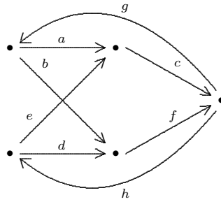
FIGURE 10. The quiver of \text{End}_{\mathcal{C}}(T')^{\text{op}}
