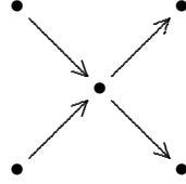
FIGURE 9. The quiver of \text{End}_{\mathcal{C}}(T)^{\text{op}}
