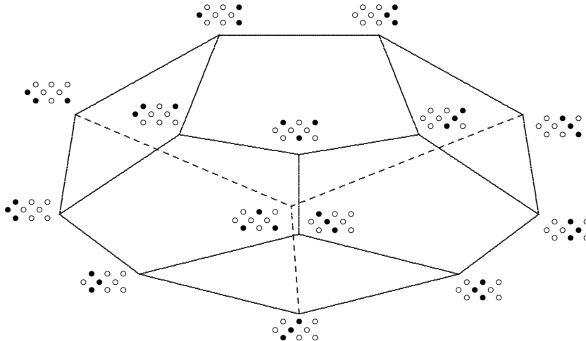
FIGURE 4. The 14 tilting sets of \mathcal{C} in type A_3
