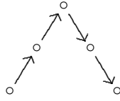
FIGURE 16. The common sub-translation quiver of the AR-quivers of \Gamma and \Gamma'
