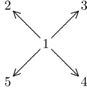
FIGURE 8. A quiver of type \widetilde{D}_4
