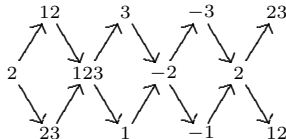
FIGURE 3. The labelled AR-quiver of \mathcal{C} in type A_3
