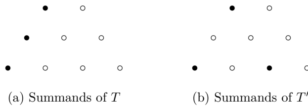
FIGURE 14. Two basic tilting objects of \mathcal{C} in type A_3
