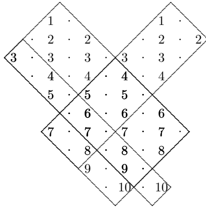
Figure 12: Configuration of all 4 rectangles.
