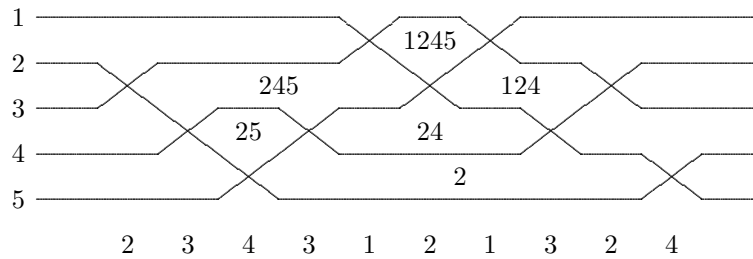
Figure 4: A chamber diagram.
