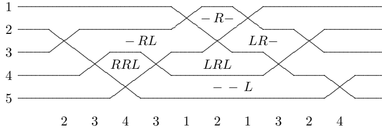
Figure 7: Partial quivers for s_2s_3s_4s_3s_1s_2s_1s_3s_2s_4 .
