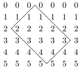
Figure 8: Drawing a (0, 2, 3, 5) -rectangle.
