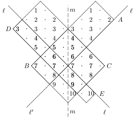
Figure 13: Configuration of all 4 rectangles with central line.
