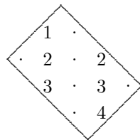
Figure 9: A (0, 2, 3, 5) -rectangle.
