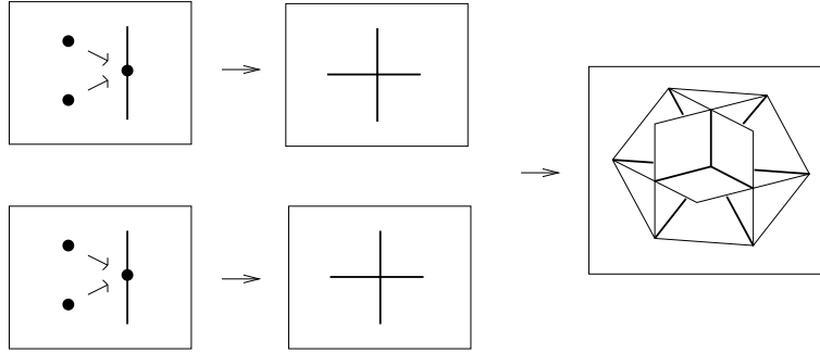
Figure 2: Binary concatenation of two simple bi-germs.
