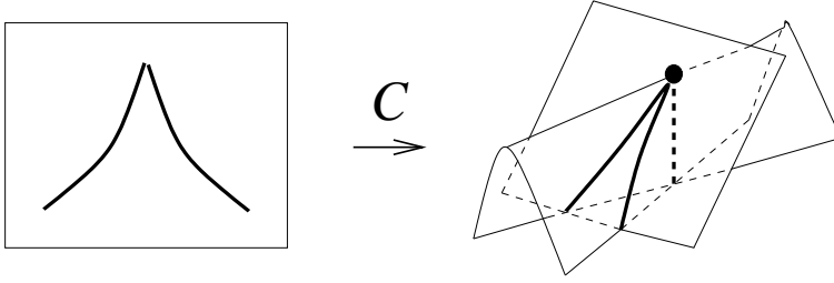
Figure 1: Monic concatenation of a cusp.
