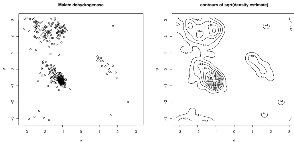
Fig. 2. Left: Ramachandran plot for Malate dehydrogenase, and Right: contour plot of estimated (sqrt) density.
