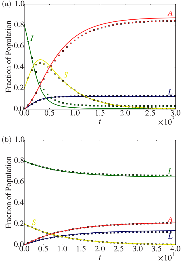
FIG. 4. (Color online) The evolution, averaged over 100 realizations, of the LISA model on an ER graph with N = 10^3 nodes, k = 10 , and I_0 = 0.8 . (a) \gamma = 0.002 , such that \gamma < (k/N)I_0 and (b) \gamma = 0.1 such that \gamma > (k/N)I_0 . Shown are the evenly distributed samples of the stochastic simulation ( \square ) and the solution of Eq. (8) (solid line). The Luddism parameter r = 0.9 .
