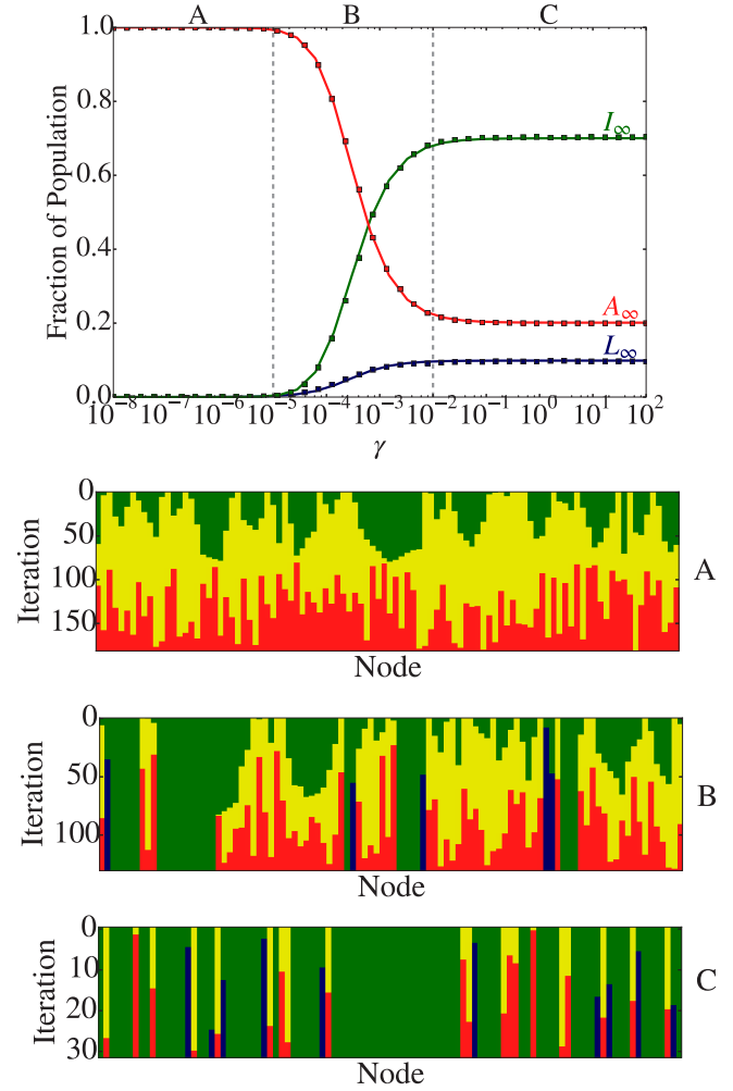
FIG. 7. (Color online) Final simulated average proportions of adopters [red (gray) \square ], ignorants [green (dark gray) \square ], and Luddites [blue (black) \square ] for varying values of \gamma , averaged over 100 simulations. Theoretical predictions using ignorant domain length (see Appendix A for details) are overlaid (solid line). Parameters are N = 1000 , r = 0.5 . Initially ignorants and susceptibles are randomly distributed, with densities I_0 = 0.8 and S_0 = 0.2 . The three regimes discussed in the text are separated by dashed lines corresponding to regions where (2/N)I_0 \ll \gamma and (2/N)I_0 \gg \gamma . Typical realizations of the model for N = 100 in each of the three regimes are given (bottom). On the vertical axis the iteration corresponds to a single step of the Gillespie algorithm, with one reaction taking place per iteration.
