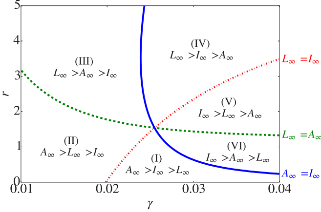
FIG. 6. (Color online) The mean-field steady-state predictions (9) over the parameter space (\gamma, r) for k/N = 0.025 and I_0 = 0.9 . The contours L_\infty = I_\infty , L_\infty = A_\infty , and I_\infty = A_\infty split the domain into six regions which characterize the innovation (see main text).
