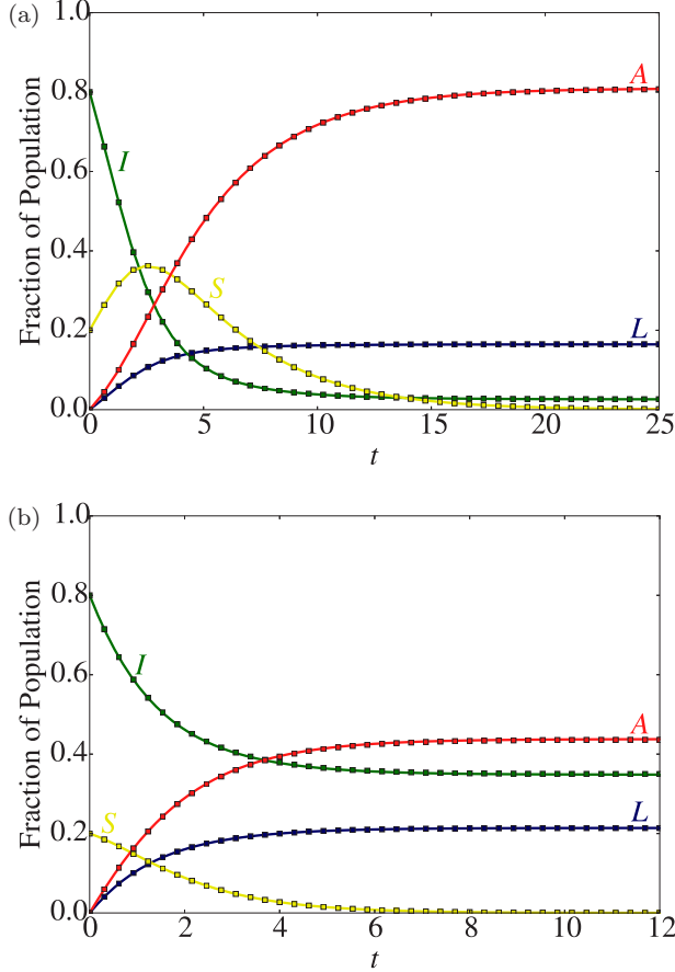
FIG. 2. (Color online) Evolution of a realization of the LISA model on a complete graph of 10^6 nodes with I_0 = 0.8 and Luddism parameter r = 0.9 . (a) \gamma = 0.3 (extensive adoption); (b) \gamma = 1 (sparse adoption). Evenly distributed samples of the stochastic simulation ( \square ) are indistinguishable from the solution of Eq. (1) (solid line). The completion times for (a) and (b) are 60 and 17, respectively.
