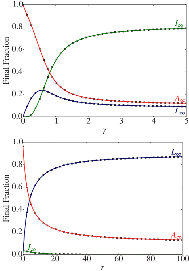
FIG. 3. (Color online) Dependencies of the final-state densities L_\infty , I_\infty , and A_\infty for a complete graph of 10^4 nodes and I_0 = 0.9 . In the top panel r = 0.9 while \gamma varies, whereas in the bottom panel \gamma = 0.3 while r varies. Simulations ( \square ) in complete agreement with (3) with substitution (7) (solid line).
