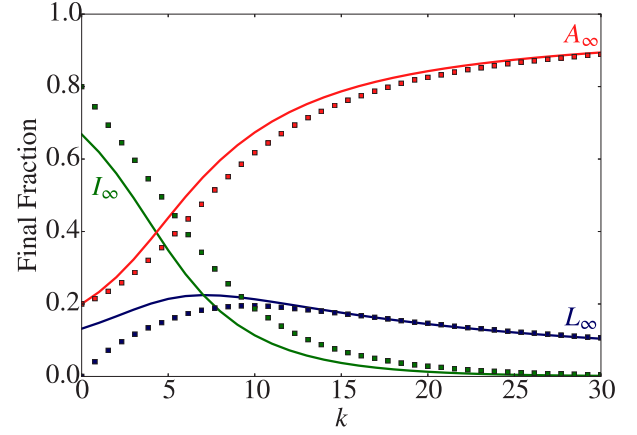
FIG. 5. (Color online) Dependence of the final densities L_\infty , I_\infty , and A_\infty on the average degree for ER graphs with N = 10^3 nodes. The simulation ( \square ) represents an average over 40 model realizations for 30 randomly generated networks. Parameters are \gamma = 0.005 , r = 0.9 , and I_0 = 0.9 . The mean-field predictions (9) (solid line) match the simulation for k \gtrsim 20 (see main text).
