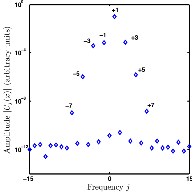
FIG. 4.1. The truncated Fourier series in time of a localized solution of the PDE (1.2), showing that e^{it} , with frequency +1, is the most important mode, that frequencies -3, -1, and +3 have similar importance, and that higher frequency modes have amplitudes at least a factor of 100 smaller. The parameter values are \mu = -0.005 , \alpha = 1 , \beta = -2 , \nu = 2 , F = 0.0579 , and C = -1 - 2.5i
