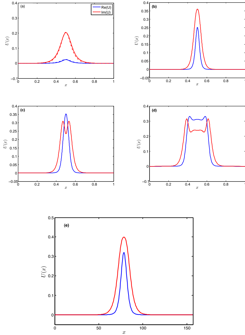
FIG. 5.1. Examples of solutions to (1.2) in the strong damping limit with \epsilon = 0.5 , F = 2.304 , \mu = -0.125 , \alpha = 1 , \beta = -2 , \nu = 2 , \omega = 1 + \nu\epsilon^2 , and C = -1 - 2.5i . The bistability region is between F_0 = 2.3083 and F_d = 1.2228 . Dotted lines in (a) represent the real (blue) and imaginary (red) parts of the analytic solution U_{loc} . The last panel is a stable solution obtained by time-stepping the PDE (1.2) at F = 1.5 , between (b) and (c).
