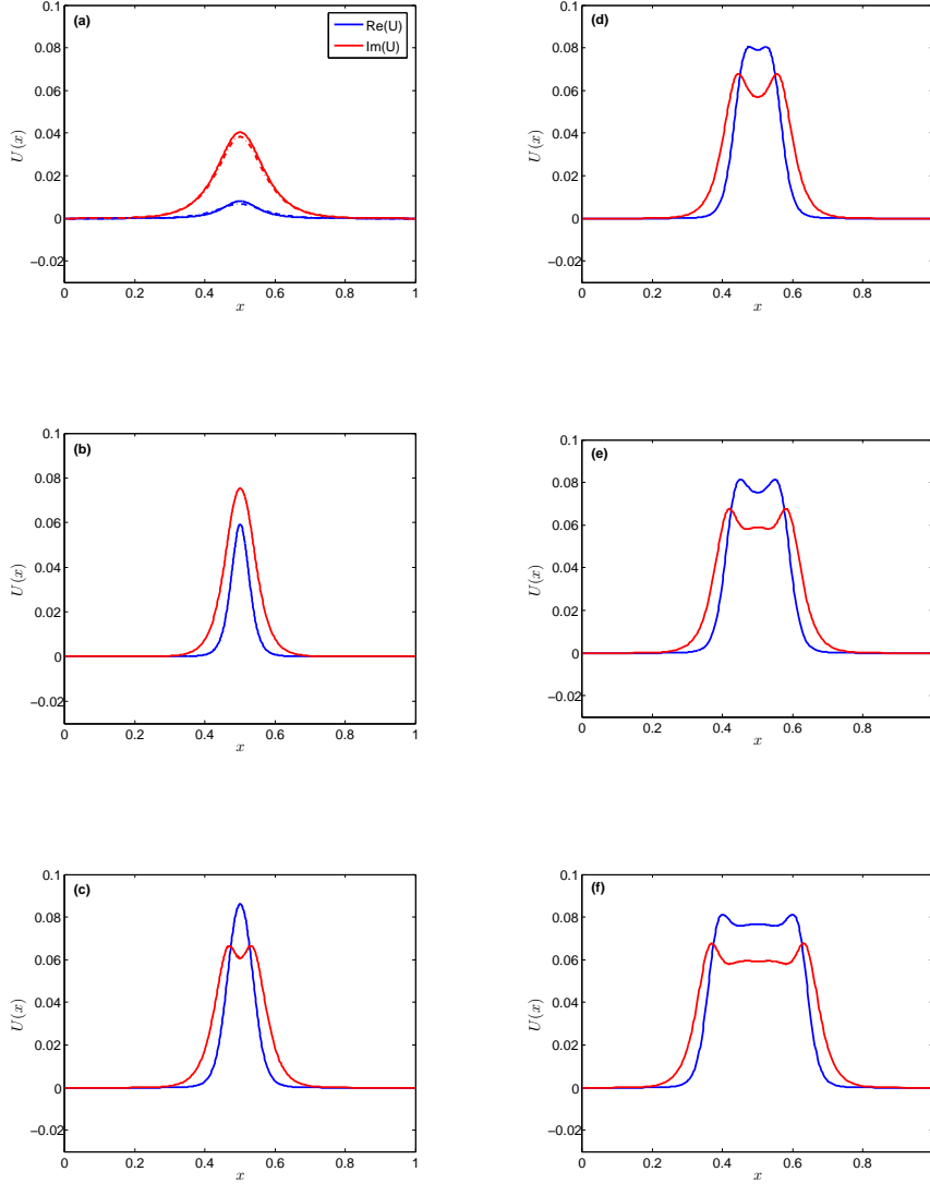
FIG. 4.6. Examples of solutions to (1.2) equation along the localized branch with \mu = -0.005 , \alpha = 1 , \beta = -2 , \nu = 2 , and C = -1 - 2.5i . Bistability region is between F_0 = 0.08165 and F_d = 0.048173 , and localized oscillons branch is between F_1^* = 0.05688 and F_2^* = 0.06001 . (a) F = 0.07499 . (b) F = 0.05699 . (c) F = 0.06015 . (d) F = 0.05961 . (e) F = 0.05976 . (f) F = 0.05975 . Dot lines represent the real (blue) and imaginary (red) parts of U_{loc} .
