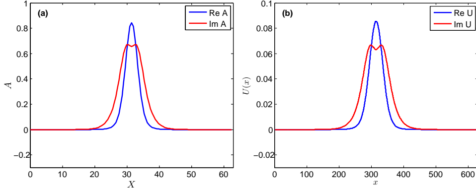
FIG. 4.2. (a) Example of a localized solution to the FCGL equation (2.5) with \mu = -0.5 , and 4\Gamma = 5.984 . (b) Example of a localized solution to the PDE model in spatial domain (1.2) with \mu = -0.5\epsilon^2 , and F = 5.984\epsilon^2 , where \epsilon = 0.1 . The solution is time-dependent and the plot is at time t = 0 . In both models \alpha = 1 , \beta = -2 , and \nu = 2 , and C = -1 - 2.5i . Note the factor of \epsilon in the scalings of the two axes.
