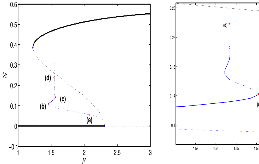
FIG. 5.2. Bifurcation diagram of the PDE with strong forcing and strong damping black lines represent the zero and flat states, and blue lines represent oscillons. The parameters as in Figure 5.1. Example solution at the points labelled (a)-(d) are in Figure 5.1.
