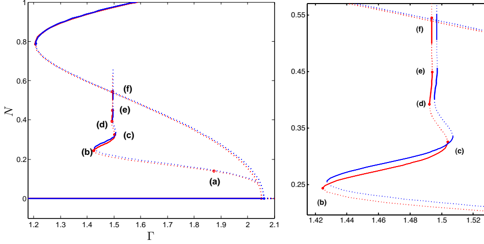
FIG. 4.5. The red curves correspond to bifurcation diagram of the PDE model and the blue curves correspond to the FCGL equation. Solid (dashed) lines correspond to stable (unstable) solutions. For the PDE we use F = 4\epsilon^2\Gamma . Parameters are otherwise as in Figure 4.2. Example solutions at the points labeled (a)-(f) are in Figure 4.6. Bifurcation point in the FCGL is \Gamma_0 = 2.06 , and in the PDE is \Gamma_0 = 2.05 . The oscillon branches terminate at the point where continuation failed.
