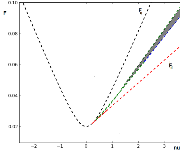
FIG. 4.4. The (\nu, F) -parameter plane of the PDE model (1.2) with \mu = -0.005 , \alpha = 1 , \beta = -2 , and C = -1 - 2.5i . Stable localized solutions exist in the shaded grey region. The dashed black line is the primary pitchfork bifurcation and the dashed red line is the saddle-node bifurcation at F_d .
