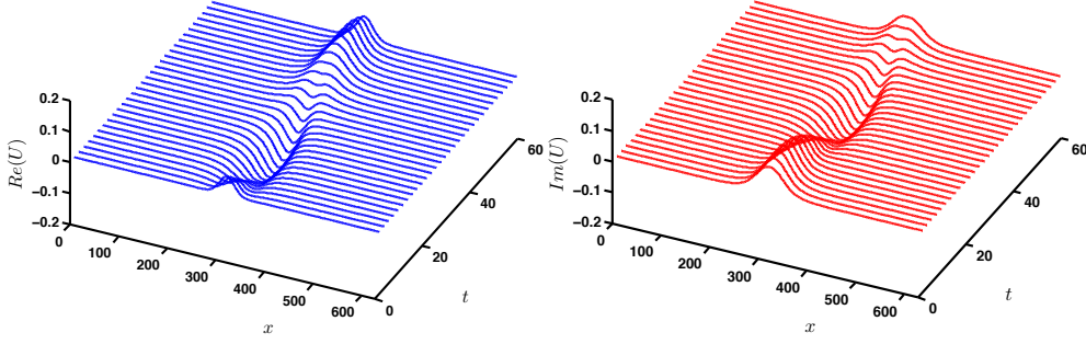
FIG. 4.7. Example of oscillon in space and time for one period 2\pi with \mu = -0.005 , \alpha = 1 , \beta = -2 , \nu = 2 , F = 0.0579 , and C = -1 - 2.5i .
