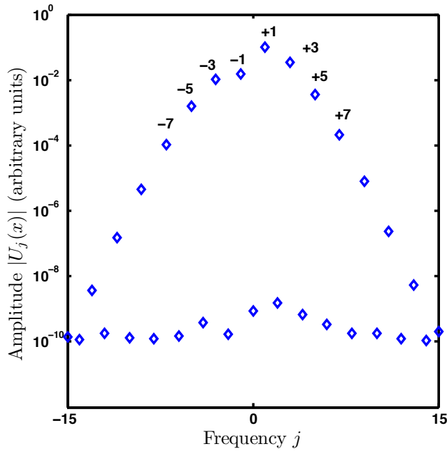
FIG. 5.3. The truncated Fourier series in time of a localized solution of the PDE (1.2) in time for one period 2\pi , showing that even with strong forcing, the modes +1 , +3 , -1 , and -3 dominate. The parameter values are the same as in Figure 5.1.
